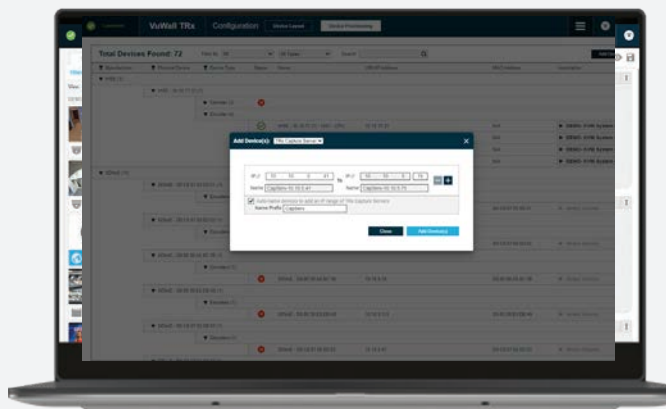
DEVICE PROVISIONING
